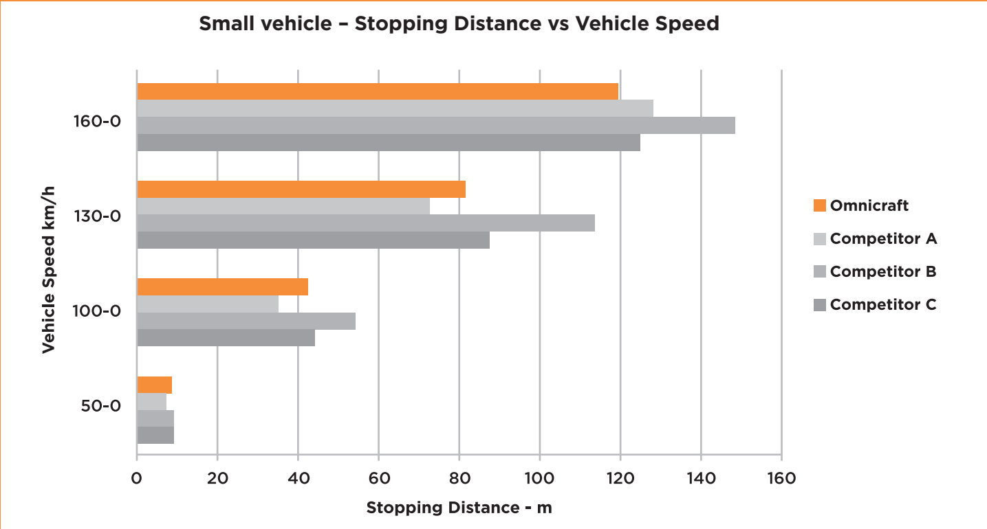
Comparison of stopping distance at various initial speeds. Omnicraft vs. Competitors (small vehicle)
