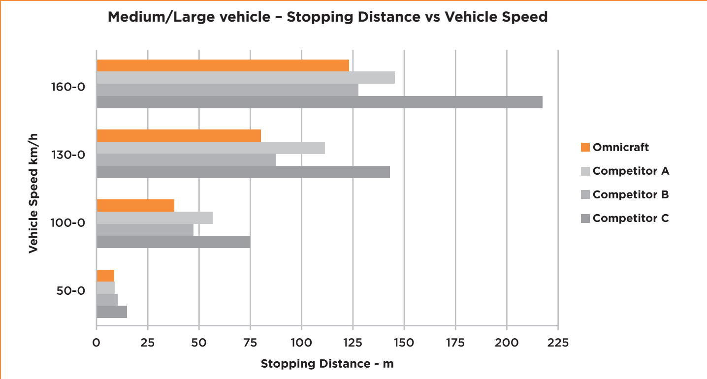
Comparison of stopping distance at various initial speeds. Omnicraft vs. Competitors (medium/large vehicle)
